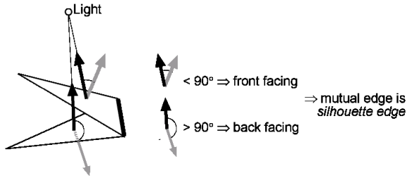
Figure 1: Silhouette edge detection.
