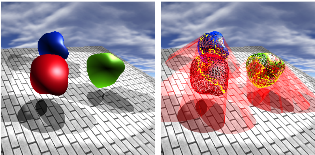
Figure 5: Scene with three light sources. The three objects are simple spheres (1000 triangles) deformed by a procedural noise shader, implemented as a vertex program. The image on the right shows the silhouette edges for one light source and the extruded shadow volumes for all lights.
